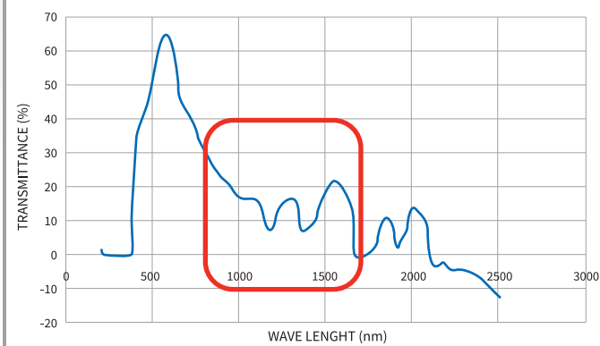
SPECTRA OF SOLARIS PMMA (ACRYLIC) 8mm
