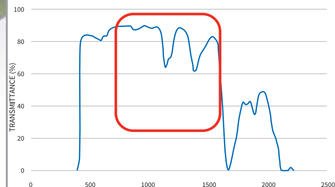
SPECTRA OF STANDARD PMMA (ACRYLIC) 8mm
