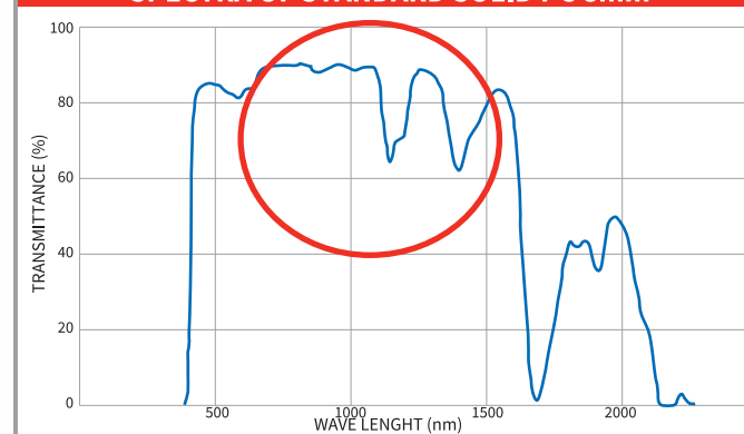
SPECTRA OF STANDARD SOLID PC 8mm
