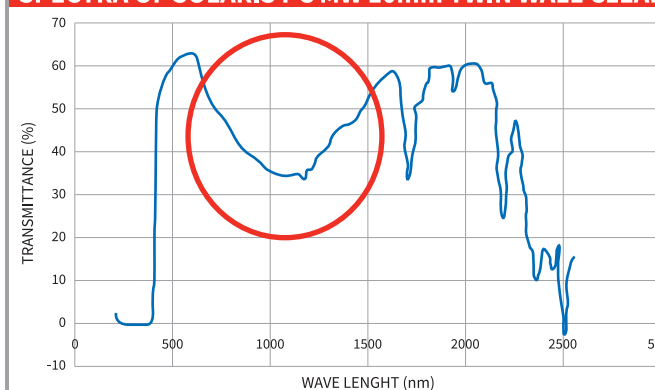
SPECTRA OF SOLARIS PC MW 10mm TWIN WALL CLEAR
